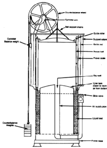
Figure 8.2: Details of Bell Prover from A.G.A. Gas Measurement Manual, Part No. 12 (1978)
