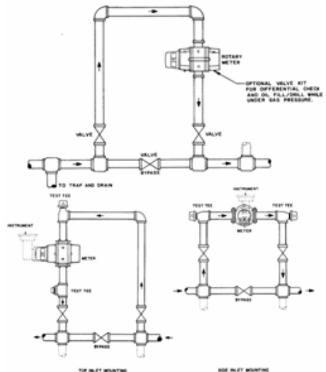
FIGURE 3. Typical Piping Arrangements
