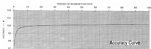
FIGURE 2. Typical Accuracy Curve
