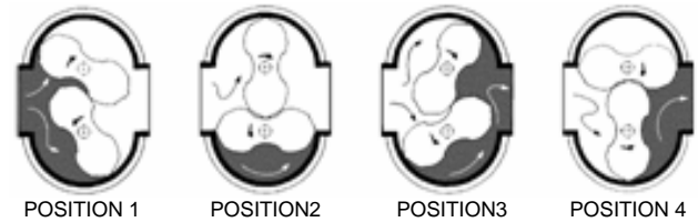
FIGURE 1. ROOTS Rotary Positive Displacement Operating Principle
