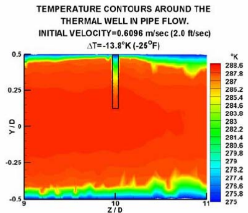
Figure 17. The effect of pipe wall temperature and velocity on thermal well temperature when the pipe wall temperature is below the flowing gas temperature. The tip of the thermal well is approximately 5°F (3°K) cooler than the gas at 0.5 ft/s. The tip of the thermal well is about equal to the flowing gas temperature at 2.0 ft/s 23 .
