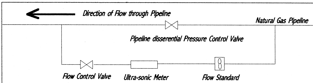
FIGURE 5. Pipeline Based Calibration Facility.
