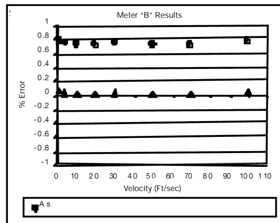
FIGURE 2. Meter "B" Results with Correction Applied.
