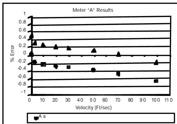
FIGURE 1. Meter "A" Results with Correction Applied.
