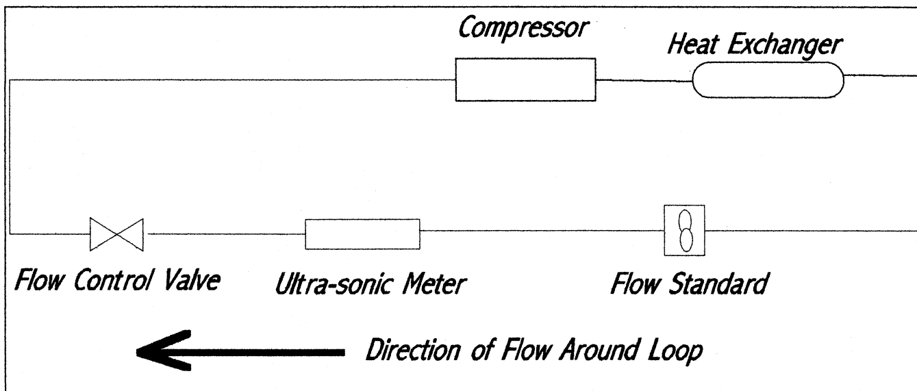
FIGURE 6. Pressurized Loop Based Calibration Facility.
