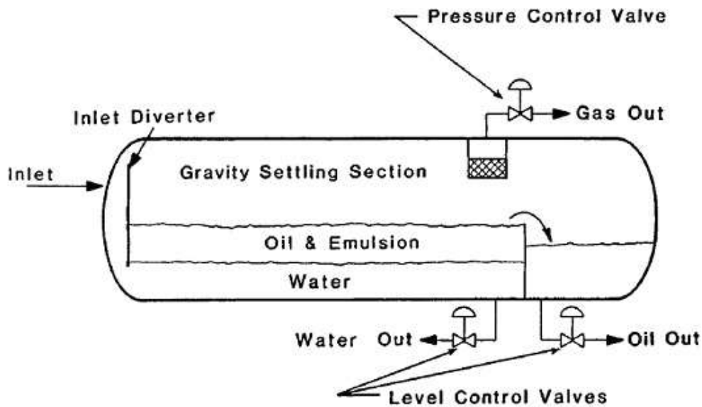
FIGURE 2. Three-Phase Separator
