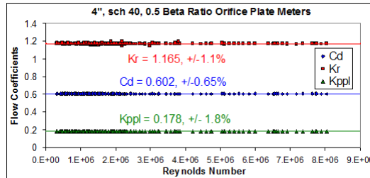
Fig 6. Combined 4”, 0.5 beta ratio DP Flow plate meter flow coefficient results.
