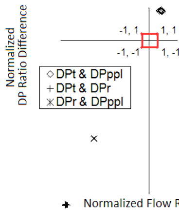
Fig 30. Rock trapped at DP Flow plate NDB plot.
