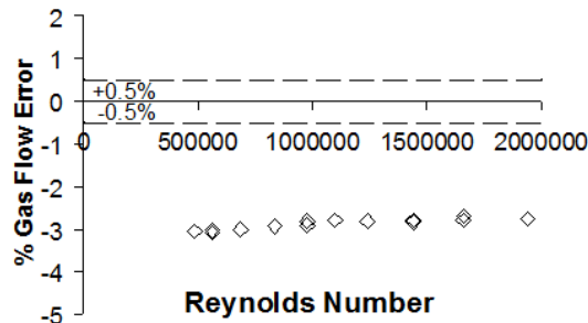
Fig 11. An DP Flow diameter flow prediction error.
