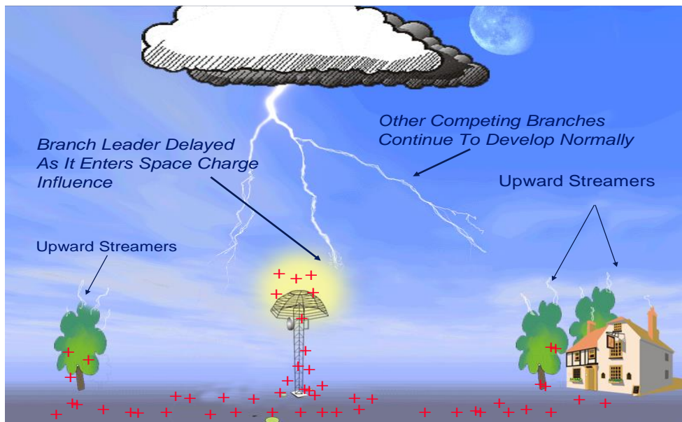
Figure 6: Reactive space charge created by the approaching lightning leader branch
