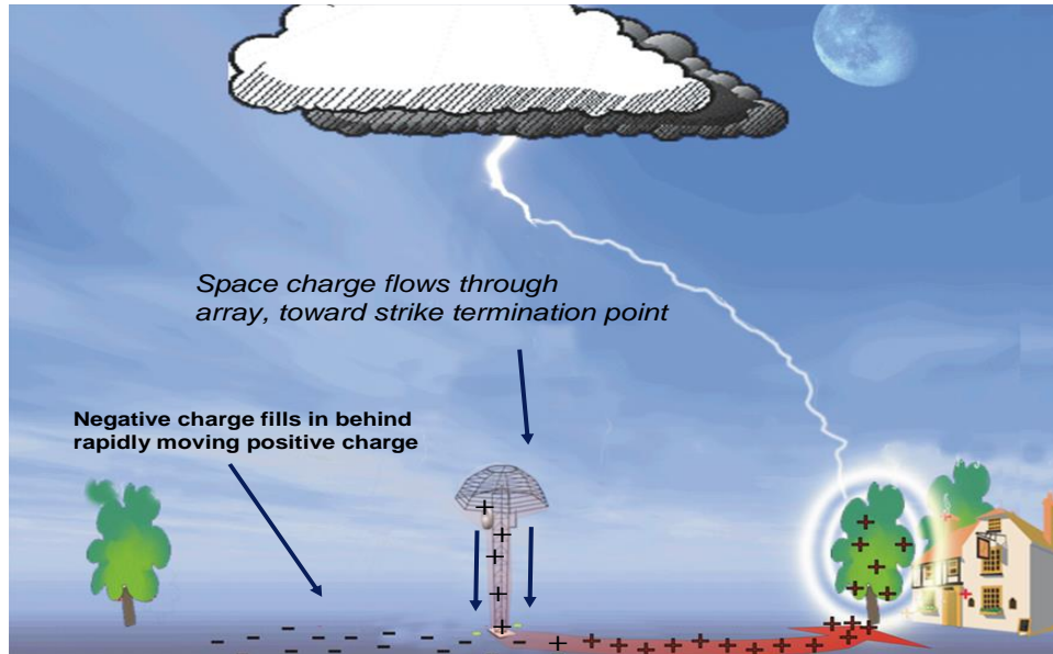
Figure 8: Charge flowing to strike terminus, others returning to neutral state
