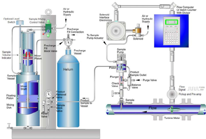
Figure 13 – Typical NGL Sampler Setup
