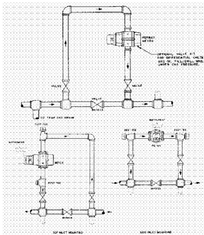
Figure 3. Typical Piping Arrangements
