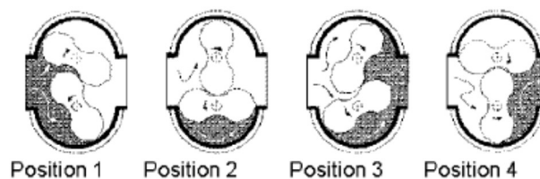
Figure 1. ROOTS Rotary Positive Displacement Operating Principle
