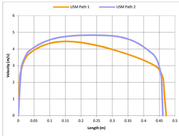
Figure 17: Velocity flow profiles for a theoretical two path Ultrasonic Meter.
