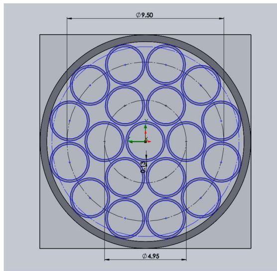
Figure 22: A CAD cutaway of an AGA3 19 tube bundle, illustrating the open flow area.
