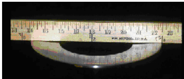
FIGURE 3. Orifice Plate Buckled by a Slug Strike
