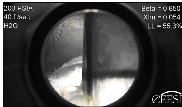
FIGURE 4. Stratified Flow Through an Orifice Plate
