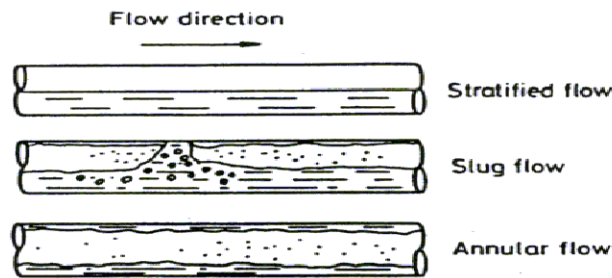
FIGURE 1. Horizontal Wet Gas Flow Pattern Maps.
