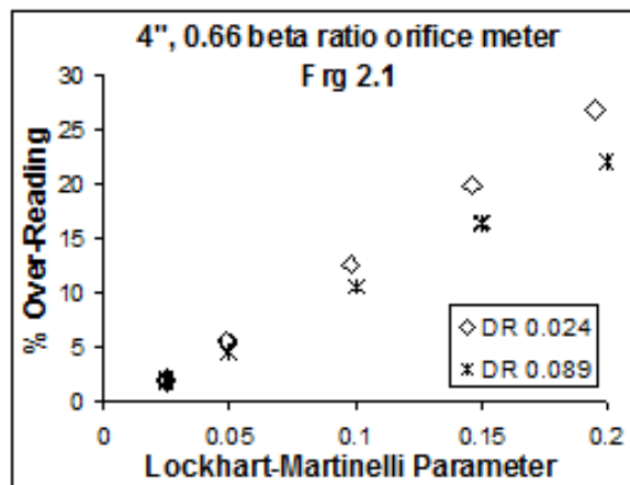
FIGURE 9. Orifice Meter Wet Gas DR Effect
