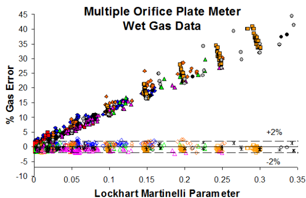
FIGURE 12. Massed Orifice Meter Wet Gas Data
