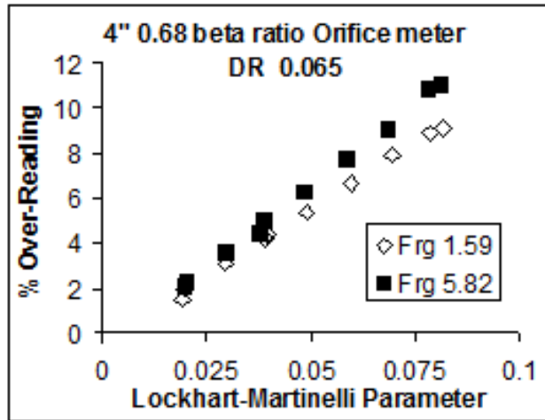
FIGURE 10. Orifice Meter Wet gas Fr g Effect
