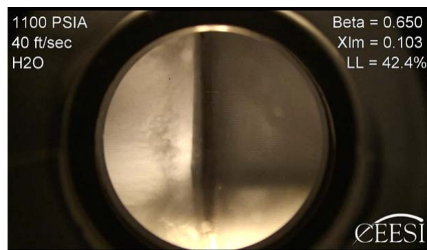
FIGURE 5. Annular Mist Flow Through an Orifice Plate
