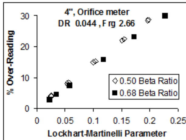
FIGURE 11. Orifice Meter Wet Gas Beta Ratio Effect
