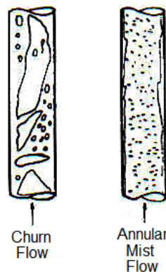
FIGURE 2. Vertical Up Wet Gas Flow Pattern Maps.
