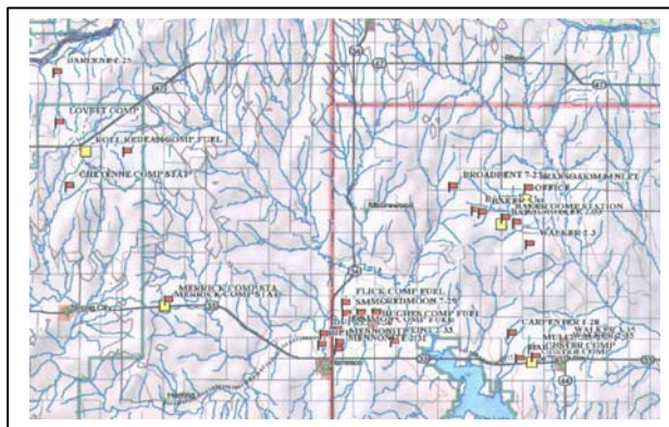
FIGURE 3. Mapping Example Showing Repeater & Slave Sites
