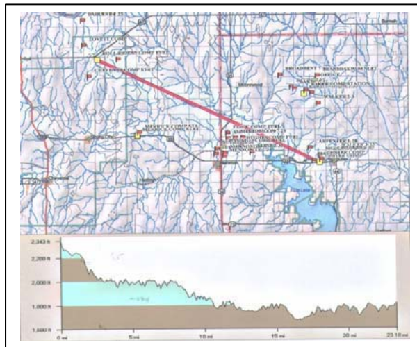
FIGURE 5. Mapping Example Showing Terrain
