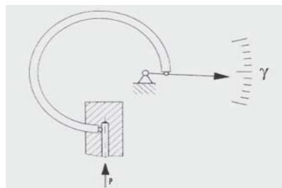
Figure 2 – Pressure Gauge Design
