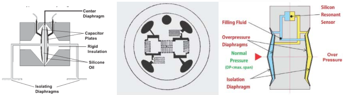
Figure 3 – Capacitance Pressure Sensor Figure 4 – Strain Gauge Sensor Figure 5 – Resonance Pressure Sensor
