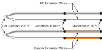
Figure 17 – Thermocouple Sensor
