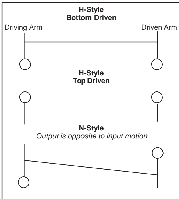
FIGURE 1. Mechanical linkage styles
