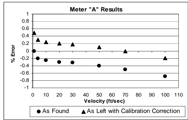
Figure 1. Meter “A” Results with Correction Applied.
