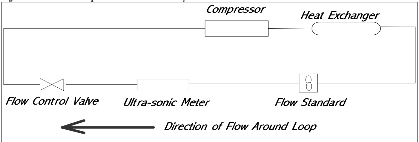
Figure 6. Pressurized Loop Based Calibration Facility.
