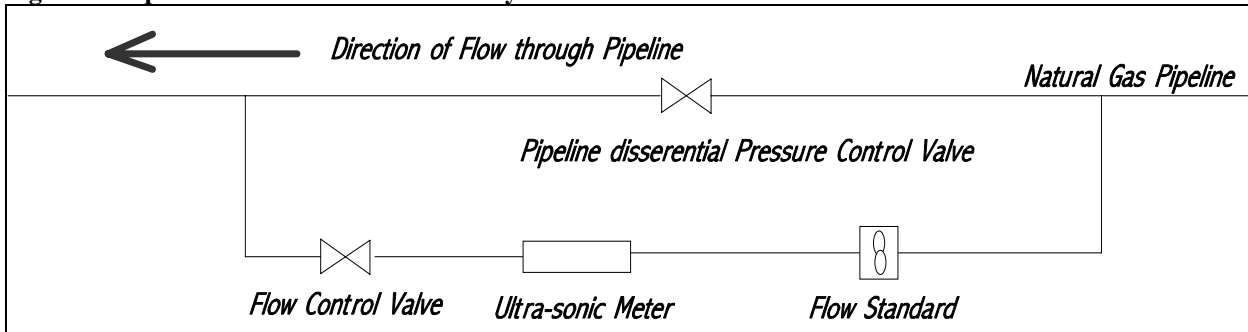
Figure 5. Pipeline Based Calibration Facility.
