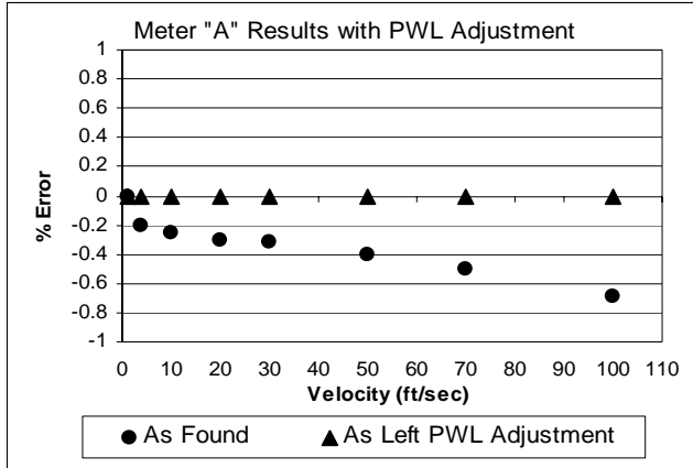
Figure 4. Meter “A” Results with PWL Adjustment Applied.
