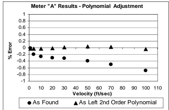
Figure 3. Meter “A” with 2 nd Order Polynomial Adjustment Applied
