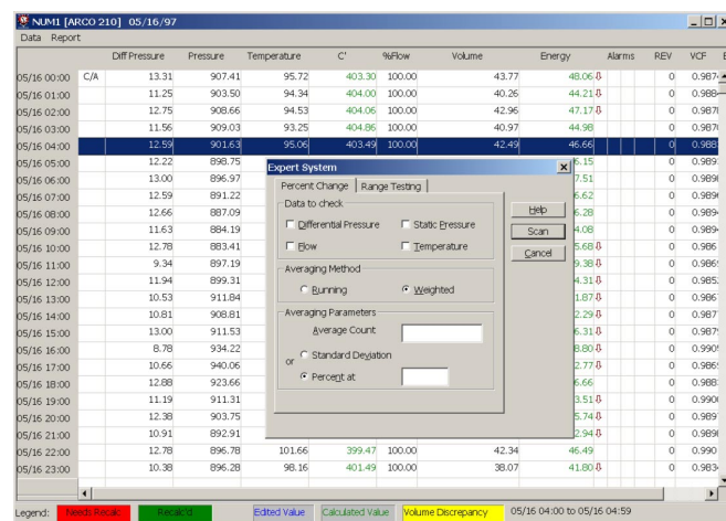
FIGURE 1. Statistical Expert System Data Scan
