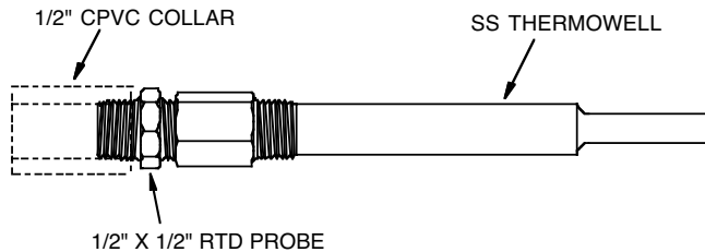
FIGURE 1. Temperature Transmitter With CPVC Coupling
