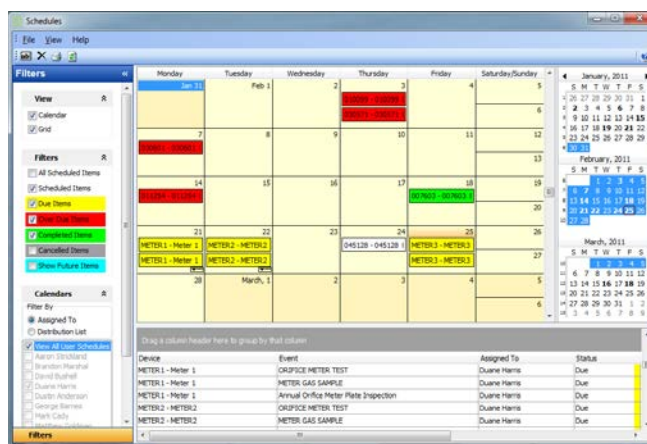
Figure 2. Calendar View
