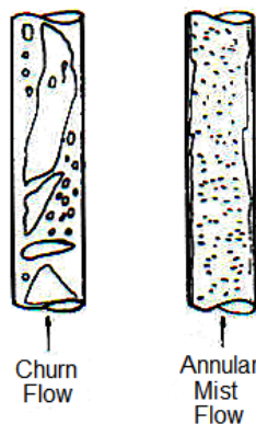
FIGURE 2. Vertical Up Wet Gas Flow Pattern Maps.
