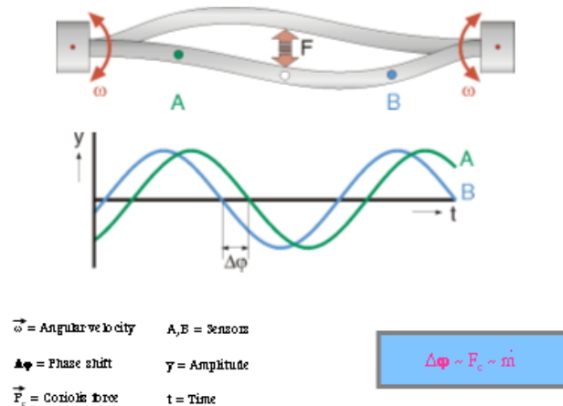
Figure 2. Coriolis Effect
