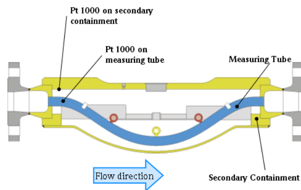
Figure 1. Coriolis Meter
