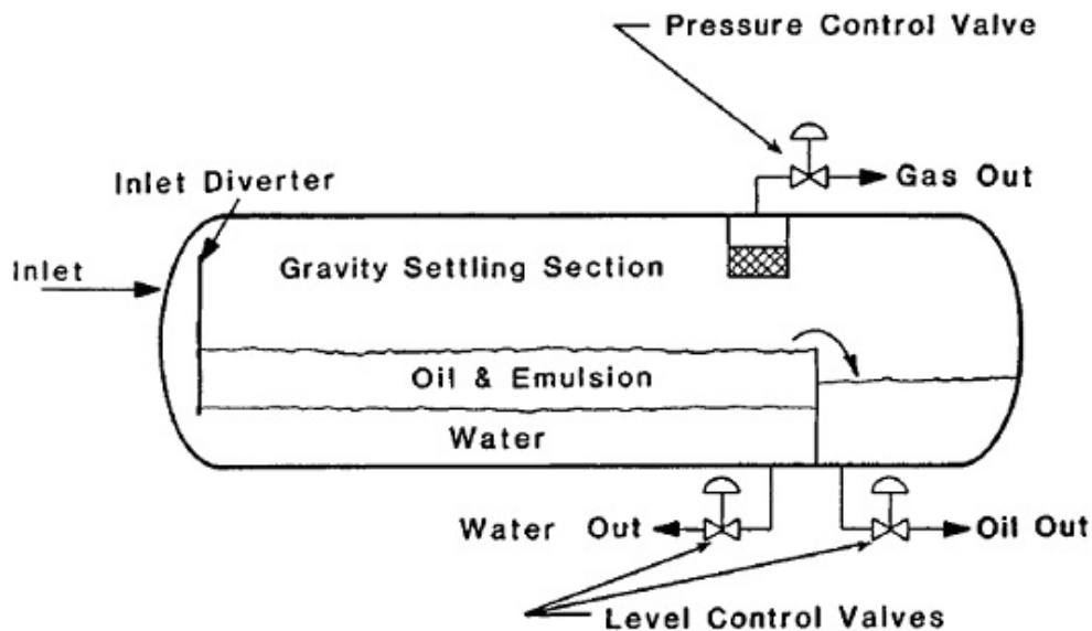
FIGURE 2. Three-Phase Separator
