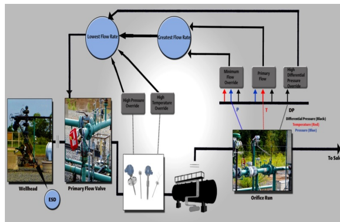
FIGURE 12. Control Scheme for Shale Gas Well Pad
