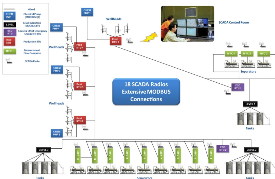
FIGURE 13. Classical Approach to Automation
