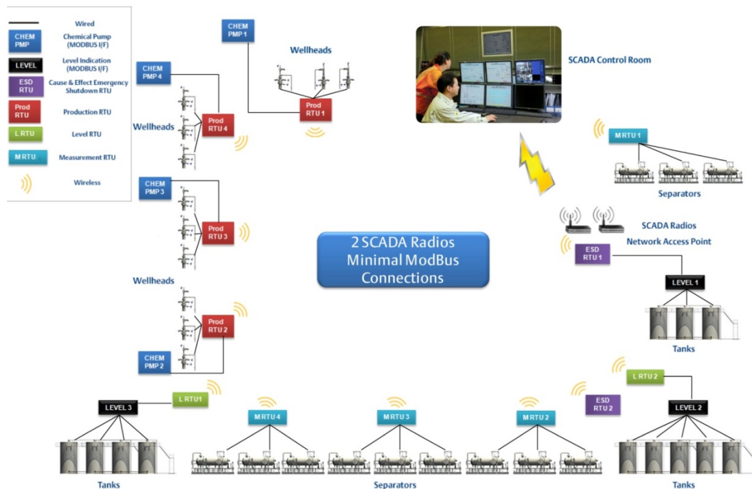
FIGURE 14. Distributed Approach to Automation
