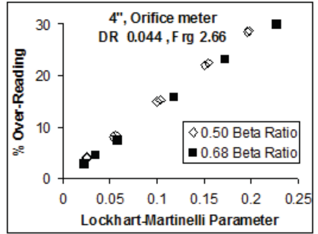
Figure 11. Orifice Meter Wet Gas Beta Ratio Effect.
