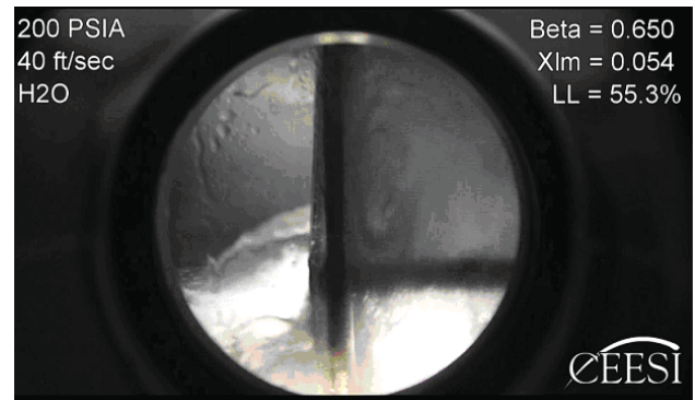
Figure 4. Stratified Flow Through an Orifice Plate.
