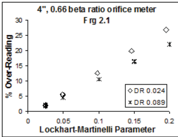
Figure 9. Orifice Meter Wet Gas DR Effect.
