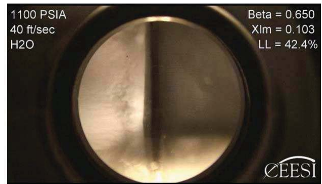
Figure 5. Annular Mist Flow Through an Orifice Plate.
