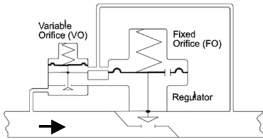
Fig. 5 Loading Type Pilot Operated Regulator
