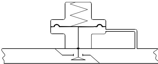
Fig. 1 Self Operated Regulator
