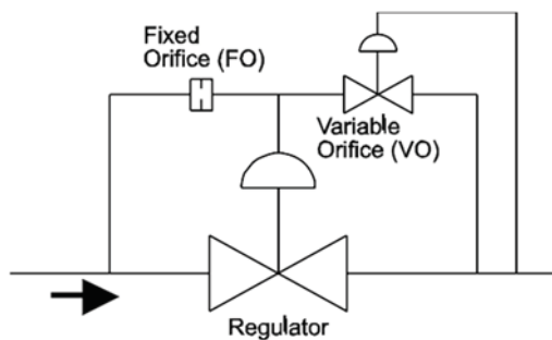
Fig. 3 Typical Pilot System
