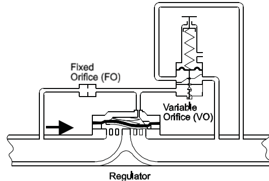
Fig. 6 Unloading Type Pilot Operated Regulator
