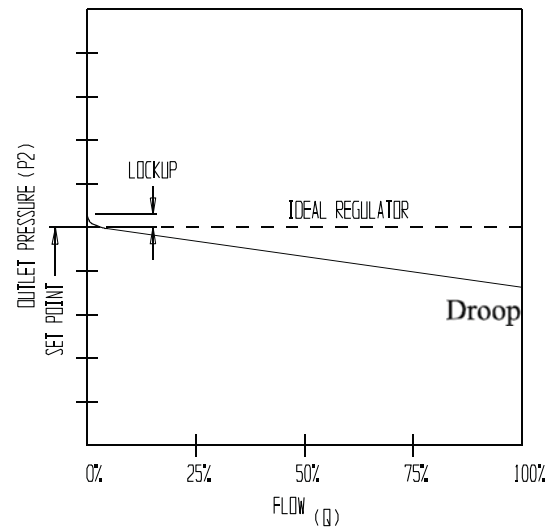
Fig 4 Typical Regulator Droop
