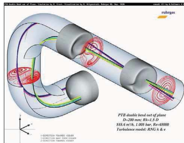
FIGURE 4. Flow Distortion Caused by Two Close-coupled 90° Elbows, 90° Out of Plane (Image courtesy of Ruhrgas)
