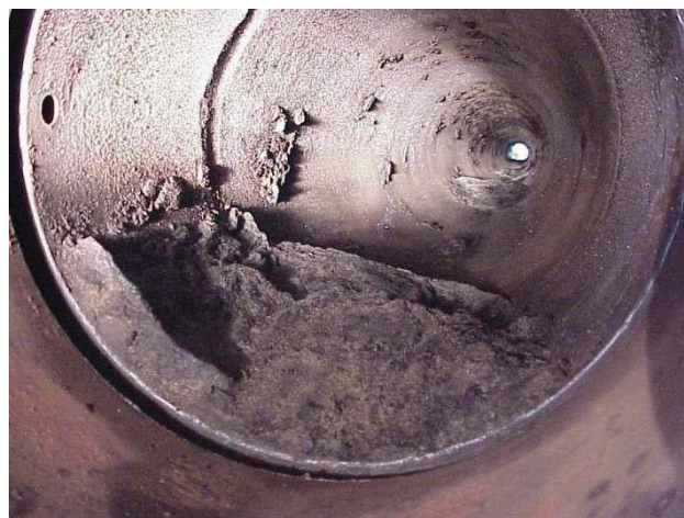
FIGURE 2. Contamination Buildup at the Plate Seat of an Orifice Flow Meter
