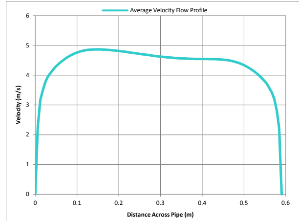
Figure 16: Average velocity profile at USM location, taken from center of pipe.
