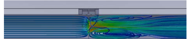
Figure 13: Visualization of velocity trajectories as flow passes through an orifice meter.
