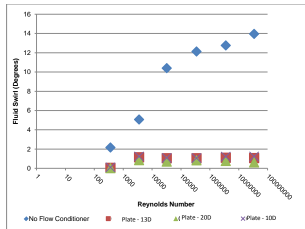
Figure 20: Showing the effectiveness of a plate based flow conditioner at eliminating swirl across a range of Reynolds numbers.
