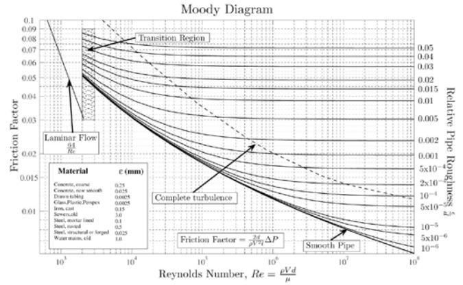
Figure 26: The Moody Diagram, used for calculating friction factor using Reynolds Number and the pipe wall roughness.
