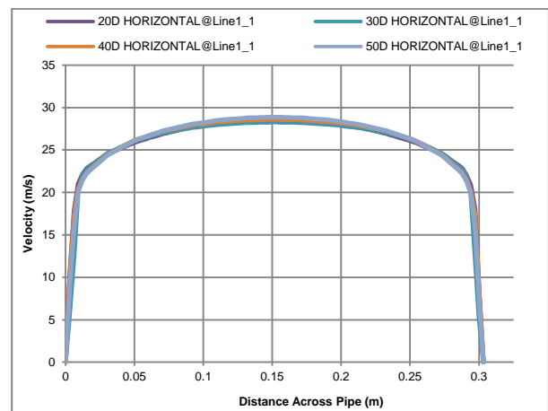
Figure 9: Flow profiles downstream of a perforated plate flow conditioner with straight pipe upstream.
