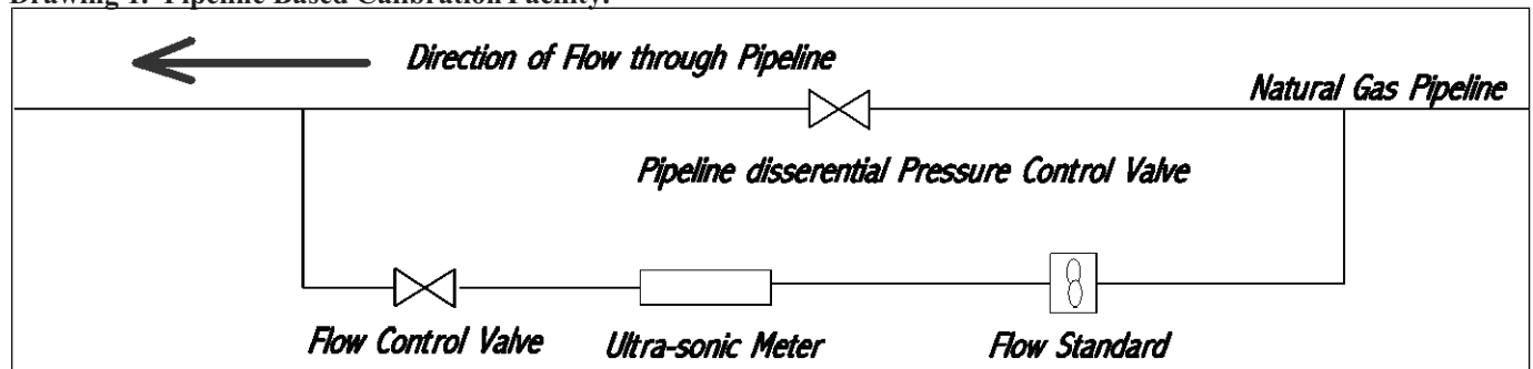
Drawing 1. Pipeline Based Calibration Facility.
