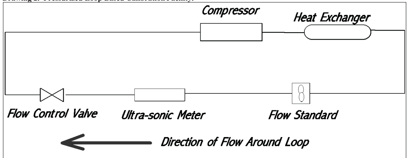
Drawing 2. Pressurized Loop Based Calibration Facility.
