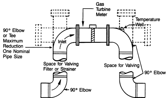
Figure 4. Close Coupled Installation
