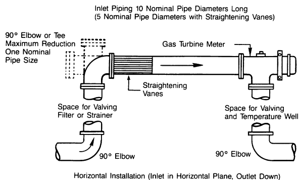
Figure 5. Angle Body Installation
