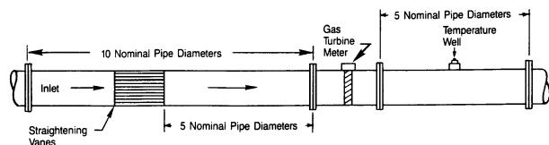
Figure 2. AGA Recommended Installation
