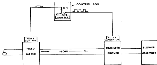
Figure 7 Transfer Proving
