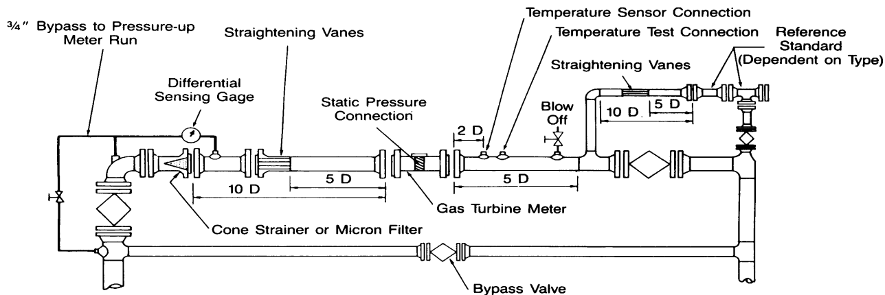
Figure 6. Turbine Meter Installation
