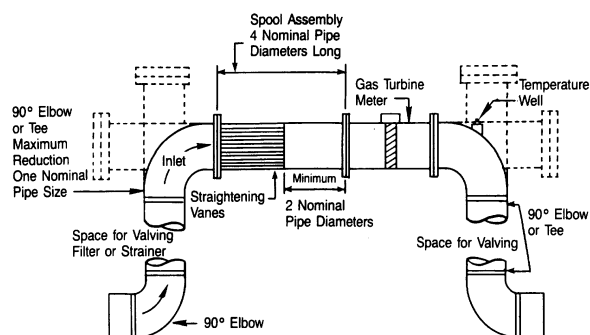
Figure 3. Short Coupled Installation
