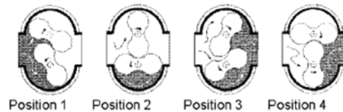
Figure 1. ROOTS Rotary Positive Displacement Operating Principle
