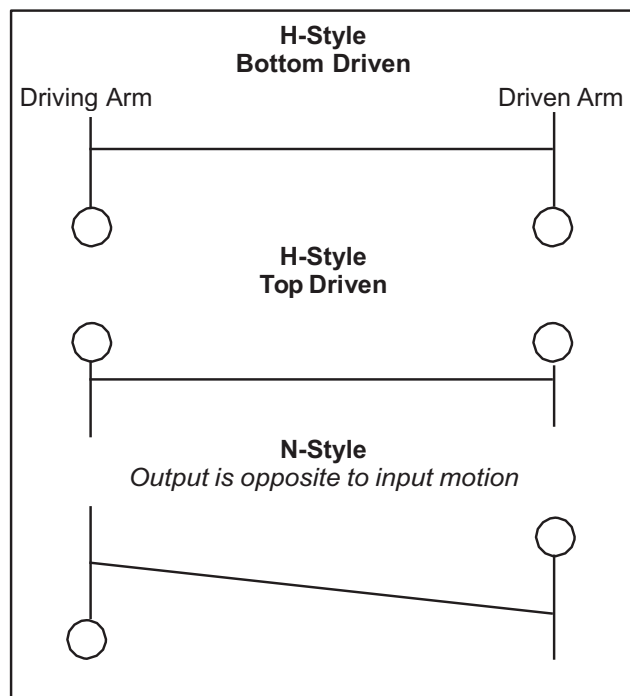
FIGURE 1. Mechanical linkage styles
