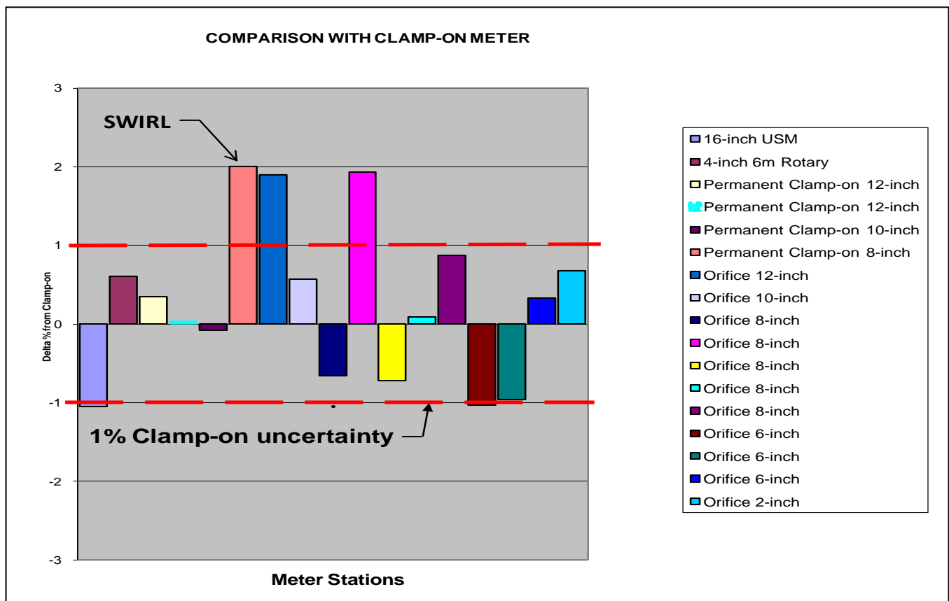
Figure XI. - FIELD COMPARISON BETWEEN CLAMP-ON AND REFERENCE METER.
