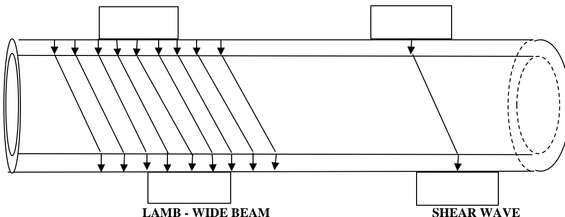
Figure I. – TRANSDUCER TYPES
