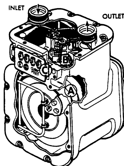
Figure 1. Diaphragm Meter
