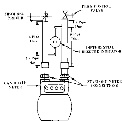
Figure 4. Test Apparatus
