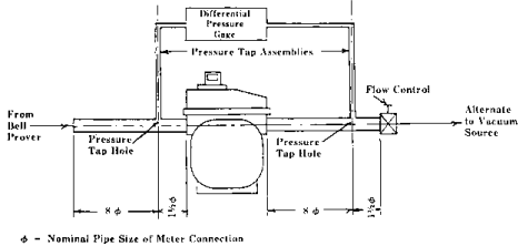
Pressure Tap Location for Side Connected Meters
