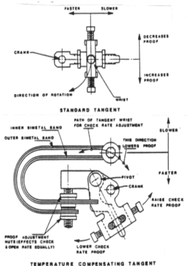
Figure 3. Tangent Adjustments
